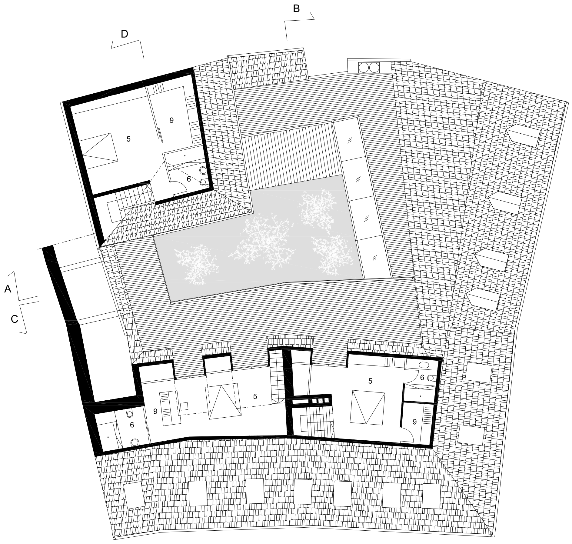
ATTIC LEVEL 2
