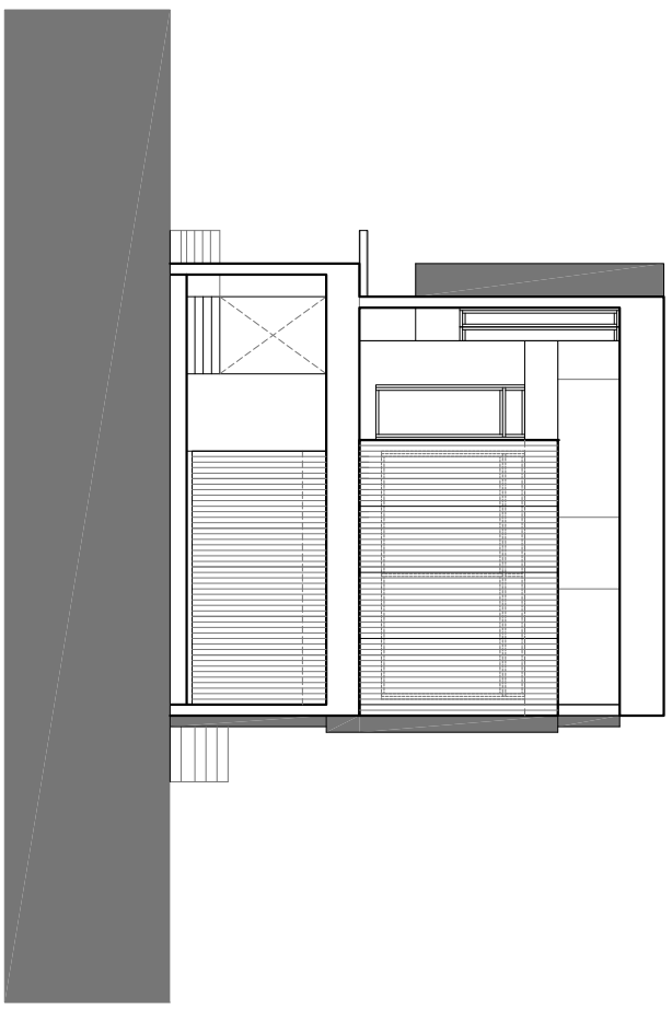
SOUTH ELEVATION
