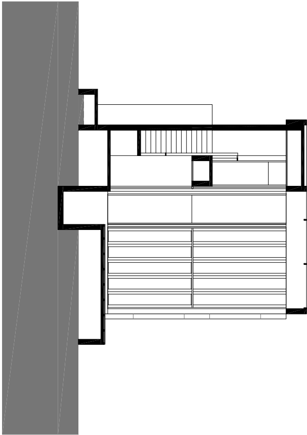
C-C SECTION
