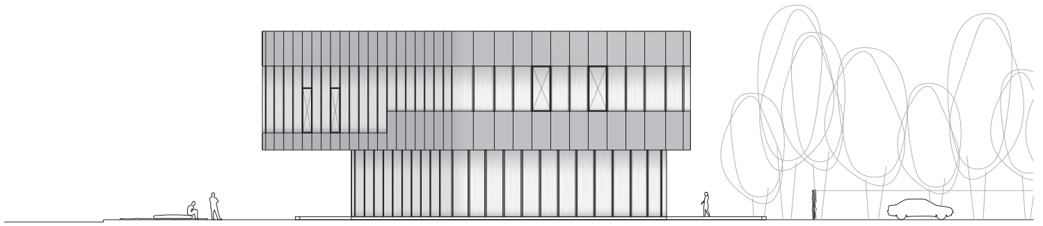
NORTH ELEVATION
