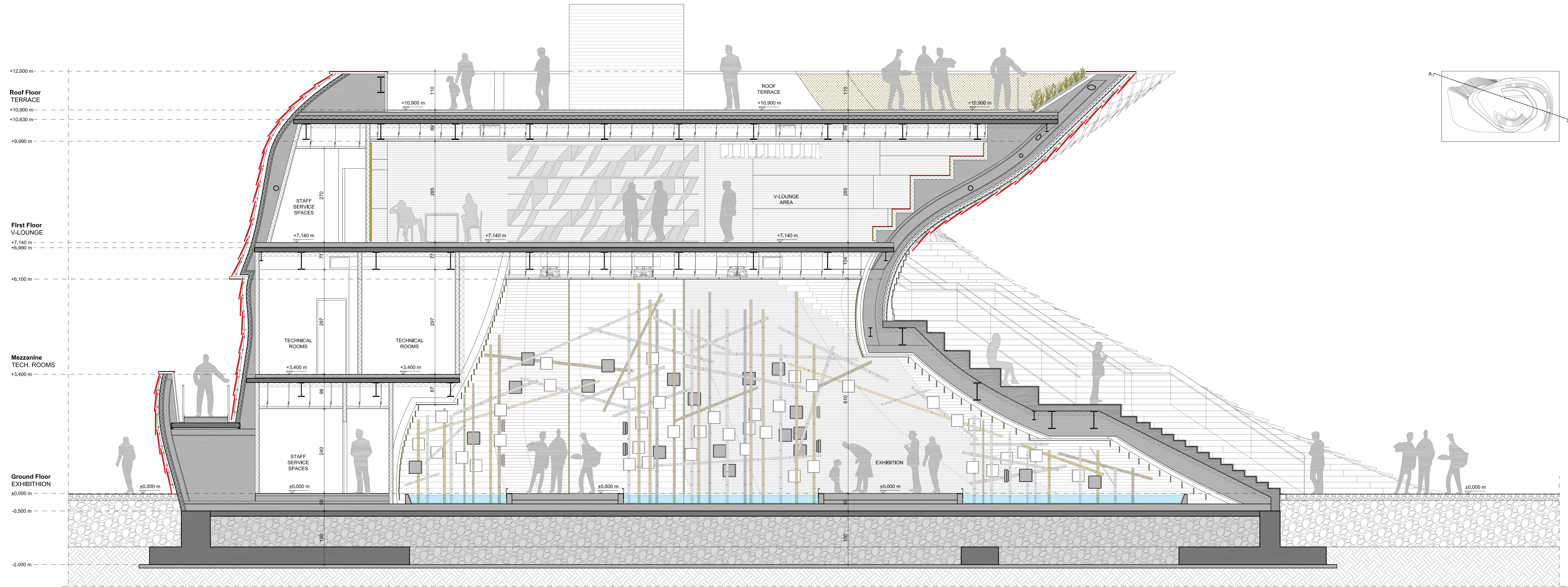
SECTION scale 1:50
