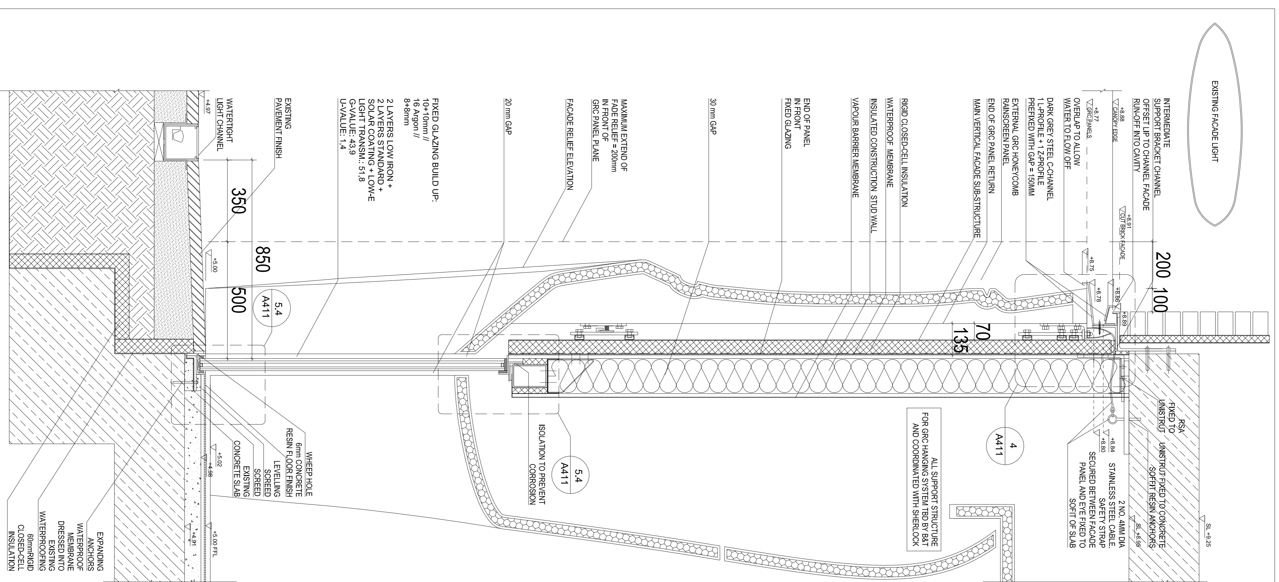
Facade Section H-H at Second Entry Fixed Glazing Section Detail Scale 1:10
