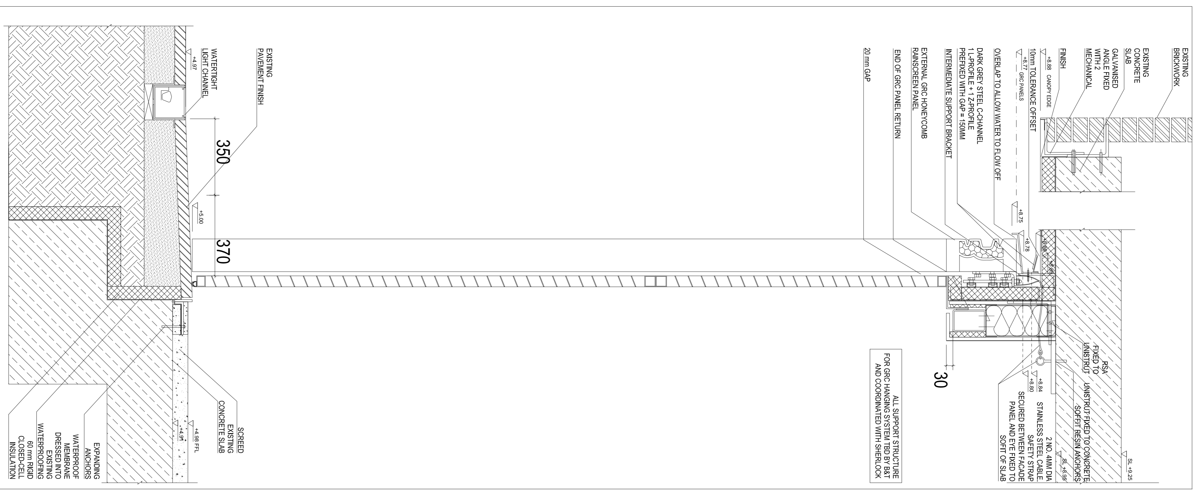
Facade Section J-J at Plant Room Door Section Detail Scale 1:10
