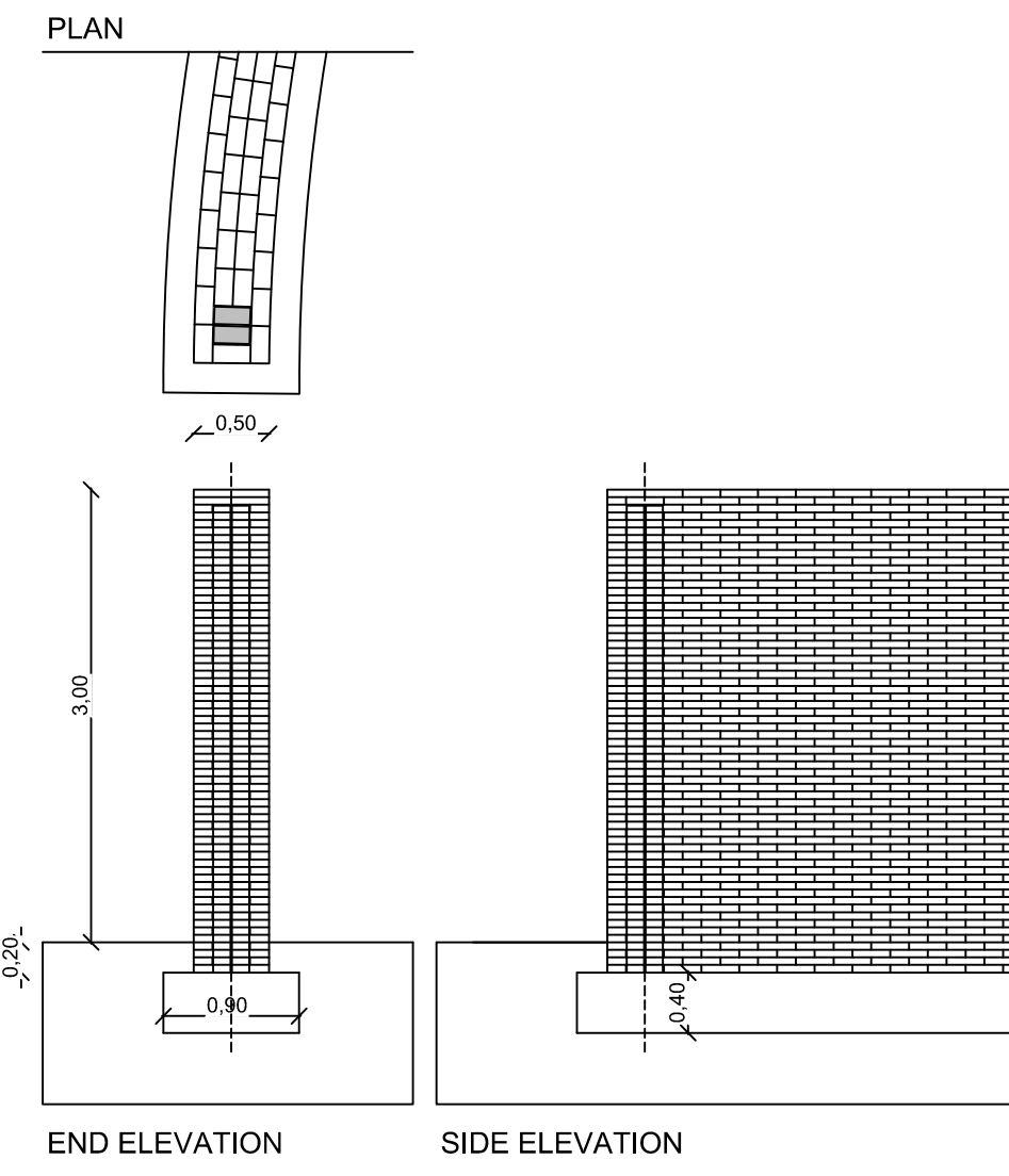
COVER BRICK DIMENSIONS
