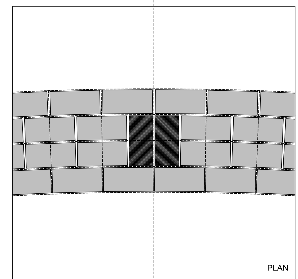
CIRCULAR WALL
